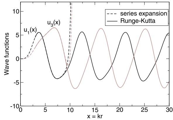
FIG. 3. (Color online) Radial wave functions u_1(x) and u_3(x) as functions of the scaled distance x = kr .
