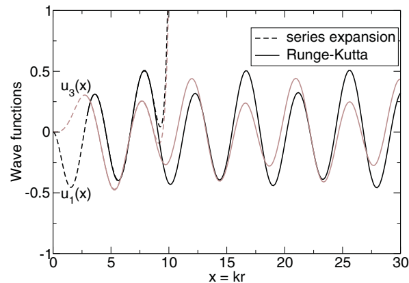
FIG. 6. (Color online) Radial wave functions u_1(x) and u_3(x) as functions of the scaled distance x = kr .
