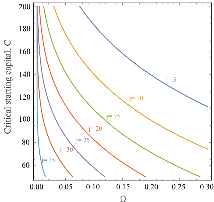
FIG. 5. The critical starting capital C (a), the corresponding average number of spins M between two catastrophic fluctuations (b), and number of successive unsuccessful spins S needed to spend the critical capital (c) as functions of \Omega calculated for the different values of the average number of bets per spin \bar{j}(N) . This calculation has been done with the probability distribution function (1).
