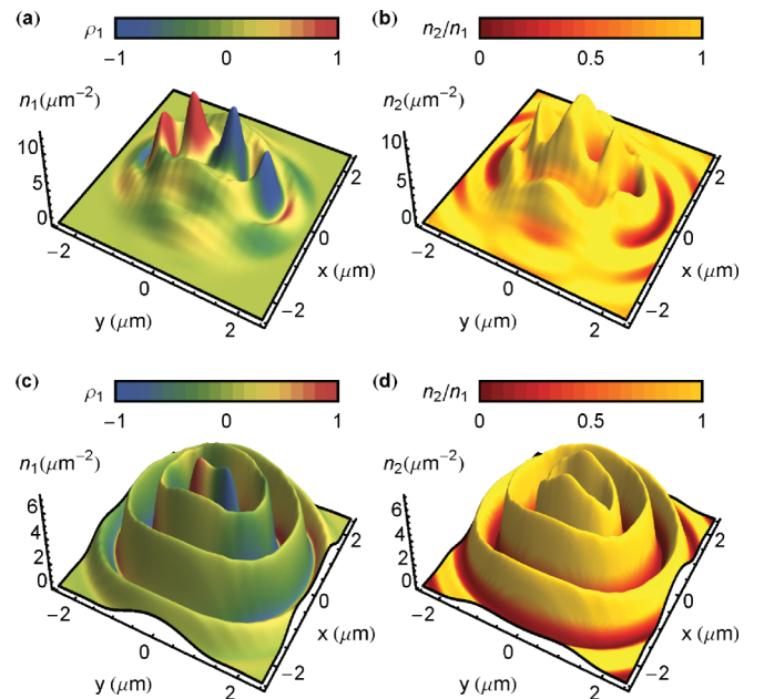
FIG. 5. (Color online) Spatial structure of four-component condensates in a strong potential trap ( m_{ex}\omega/2 = 1 \text{ μeV μm}^{-2} ). The bright (a) and dark (b) exciton intensity is shown for the case W = -0.2V_0 . The variation of the spin-polarization degree of bright excitons is shown by the colors in (a). Dark excitons have approximately zero circular polarization degree. The ratio of the dark to bright exciton density is shown by the colors in (b). (c) and (d) show the corresponding profiles for the case W = 0.2V_0 .
