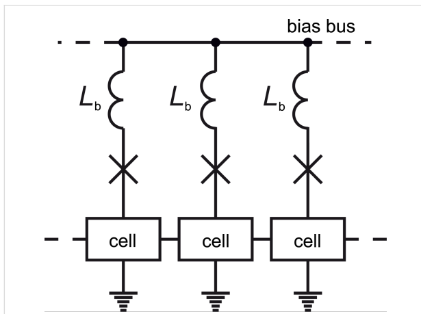
Figure 5: ERSFQ power supply scheme. L_b is the inductance limiting the bias current variation.
