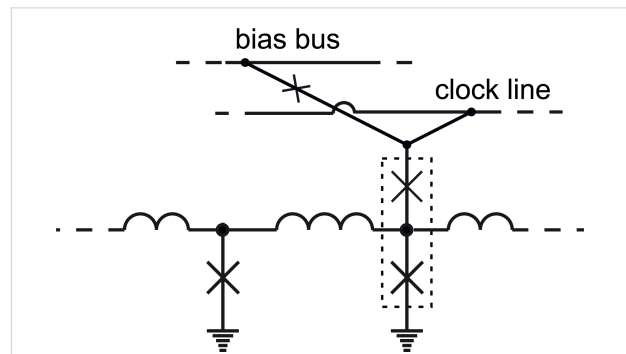
Figure 6: eSFQ power supply scheme. The dotted rectangle marks the decision-making pair.
