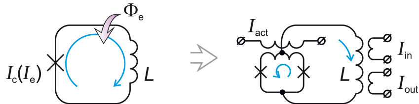
Figure 10: Notional (left) and practical (right) schematic of a parametric quantron. The cell state is conditioned by bias flux \Phi_e and current I_e controlling the critical current I_c of the Josephson junction. L is the loop inductance. In practice, the single Josephson junction is substituted with a SQUID controlled by the activation current I_{act} . I_{in}/I_{out} are input/output currents.
